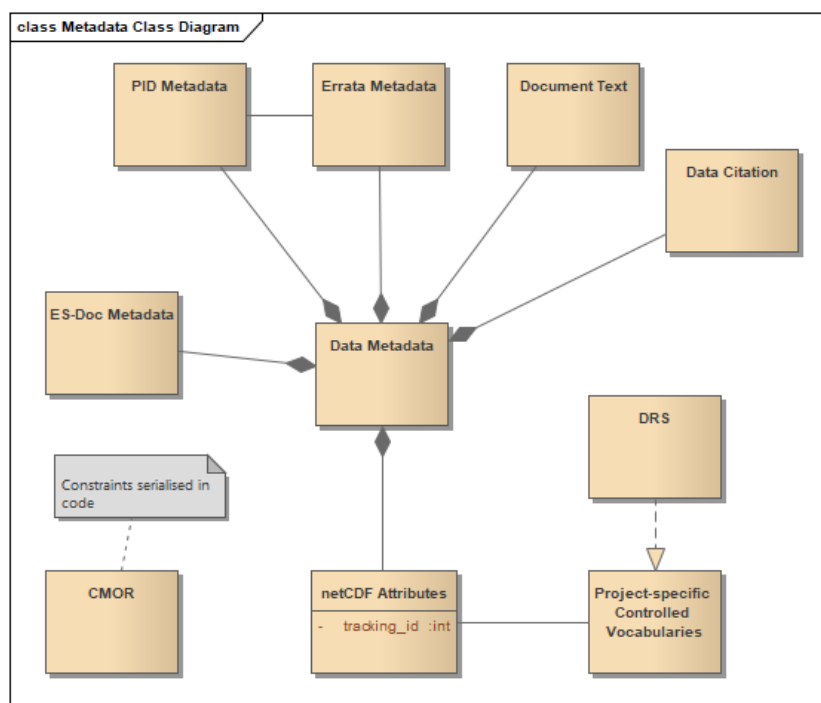
Figure 8: analysis of classes of metadata in ESGF and their relationship
